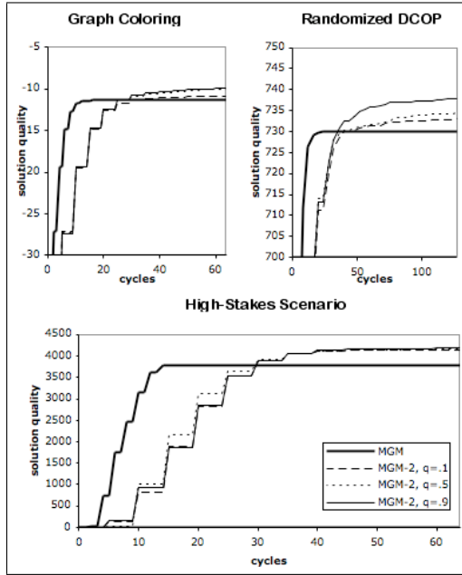
(b) Comparison of the performance of MGM and MGM-2
