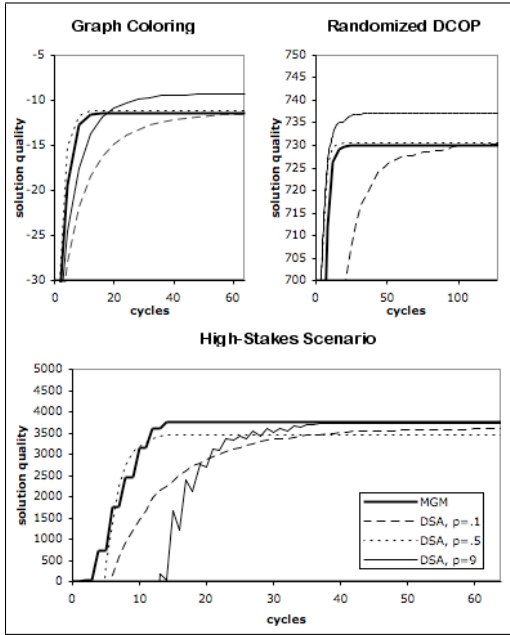
(a) Comparison of the performance of MGM and DSA
