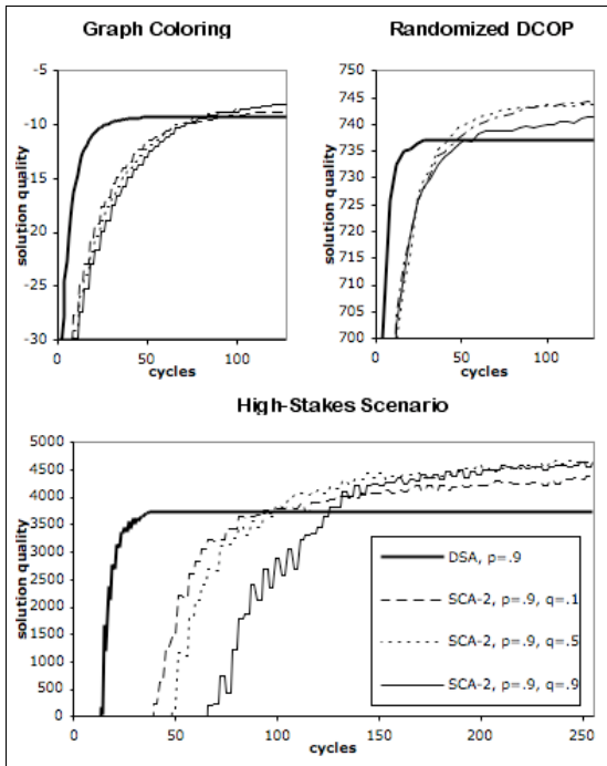
(c) Comparison of the performance of DSA and SCA-2
