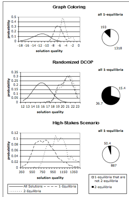
(d) Distributions of Solution Quality for X, X_E, X_{2E} and Cardinality of X_{2E} as a proportion of X_E
